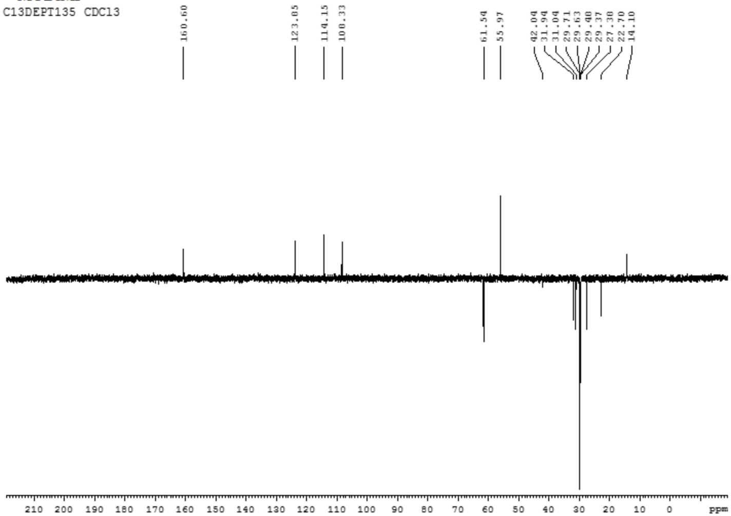
DEPT NMR spectrum 2-methoxy-6-[(octadecylimino)methyl]phenol
