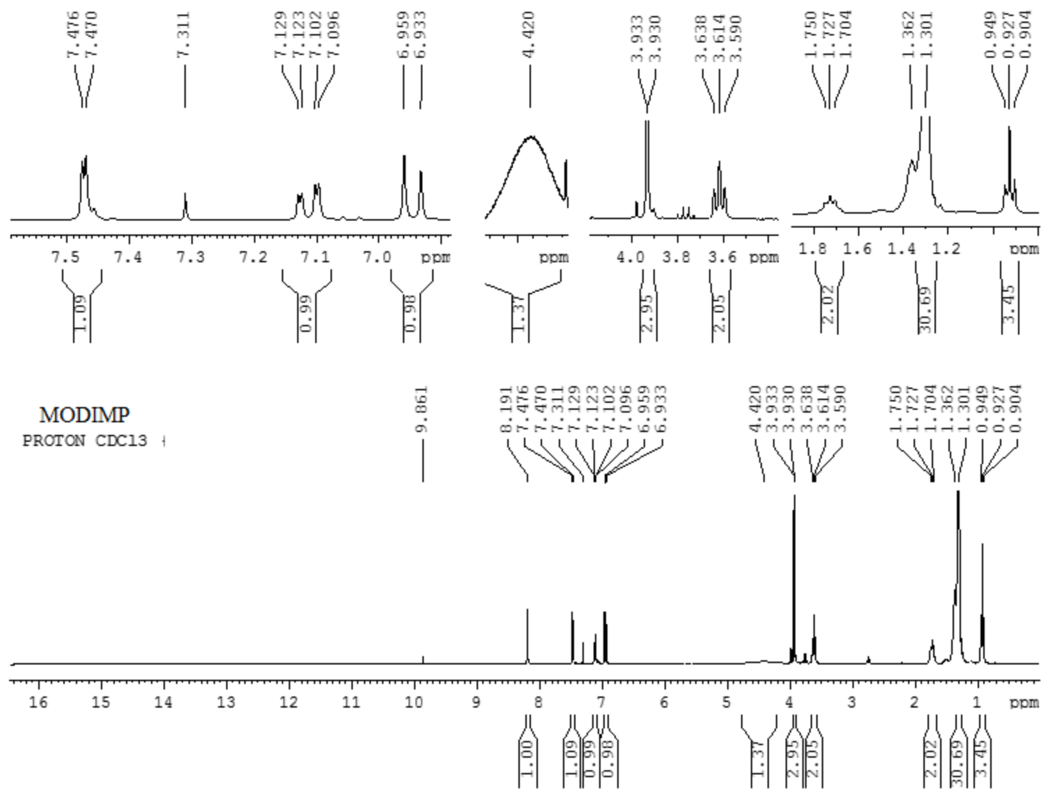
1 H NMR spectrum 2-methoxy-6-[(octadecylimino)methyl]phenol.
