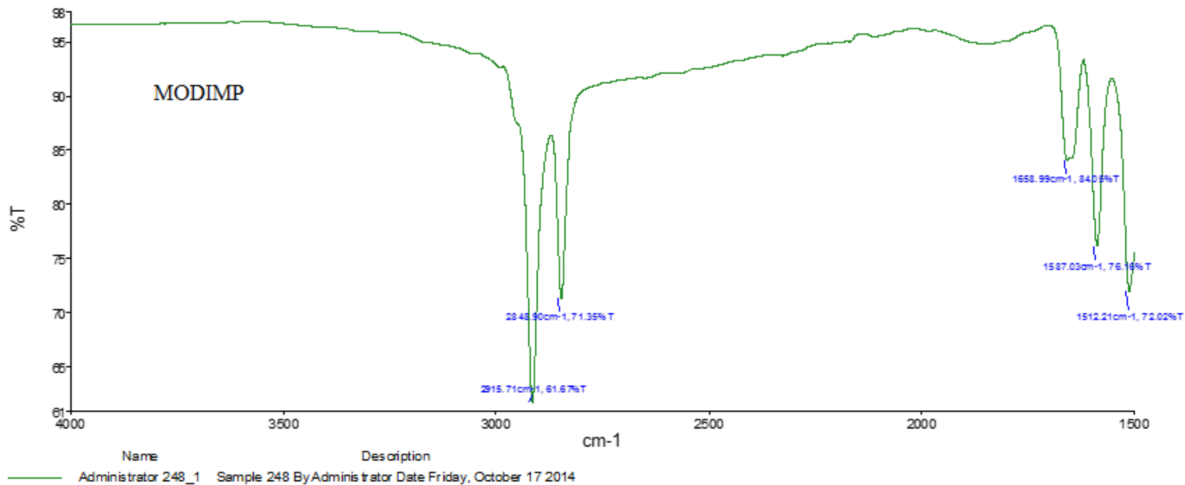
IR spectrum of 2-methoxy-6-[(octadecylimino)methyl]phenol (MODIMP)
