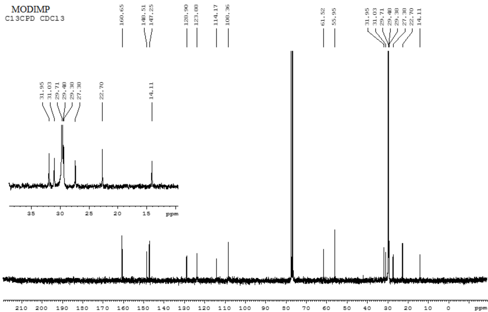
13 C NMR spectrum 2-methoxy-6-[(octadecylimino)methyl]phenol
