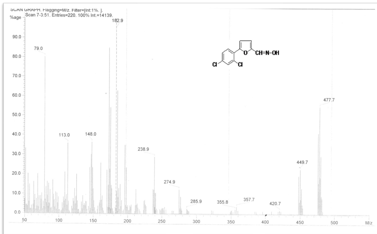
Mass spectra of 5-(2',4-dichlorophenyl) furan-2-carbaldehyde oxime: (12)
