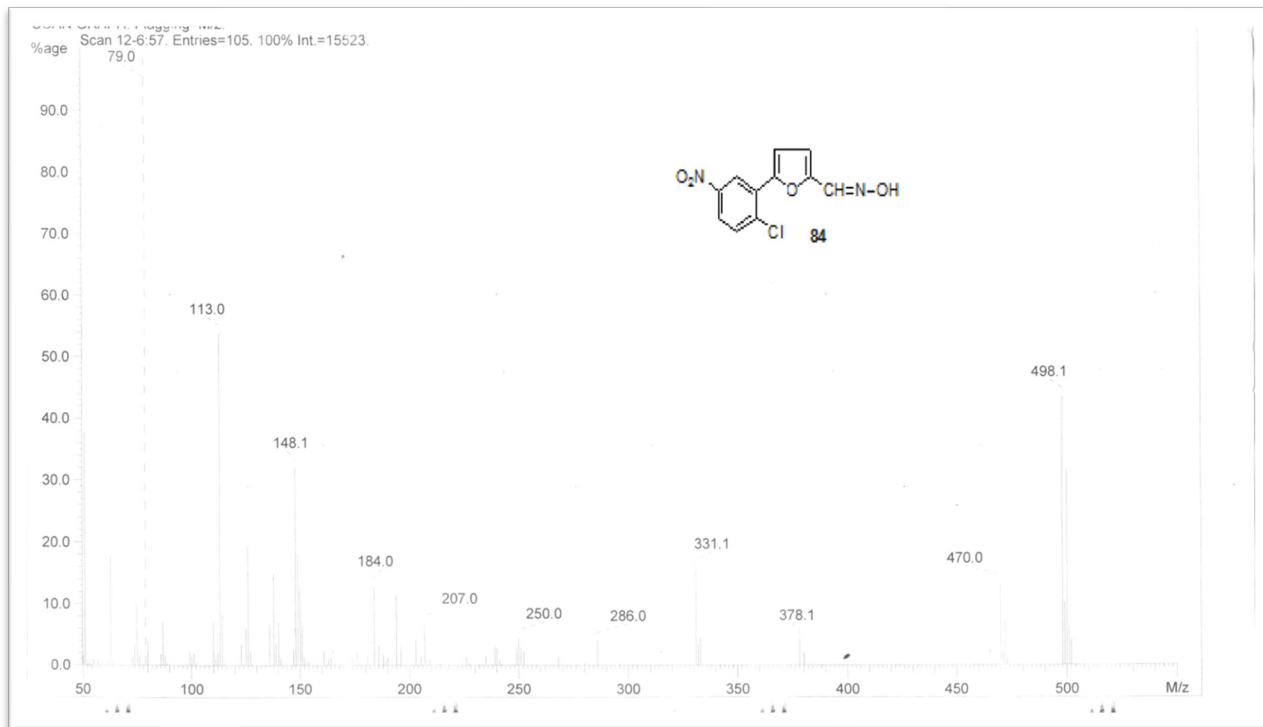
Mass spectra of 5-(2'-chloro-5'-nitrophenyl) furan-2-carbaldehyde oxime: (20)
