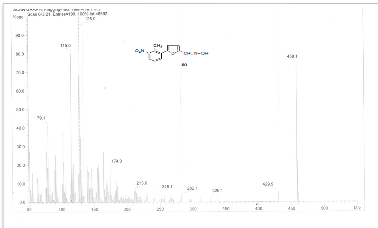
Mass spectra of 5-(2'-methyl-3'-nitrophenyl) furan-2-carbaldehyde oxime: (17)
