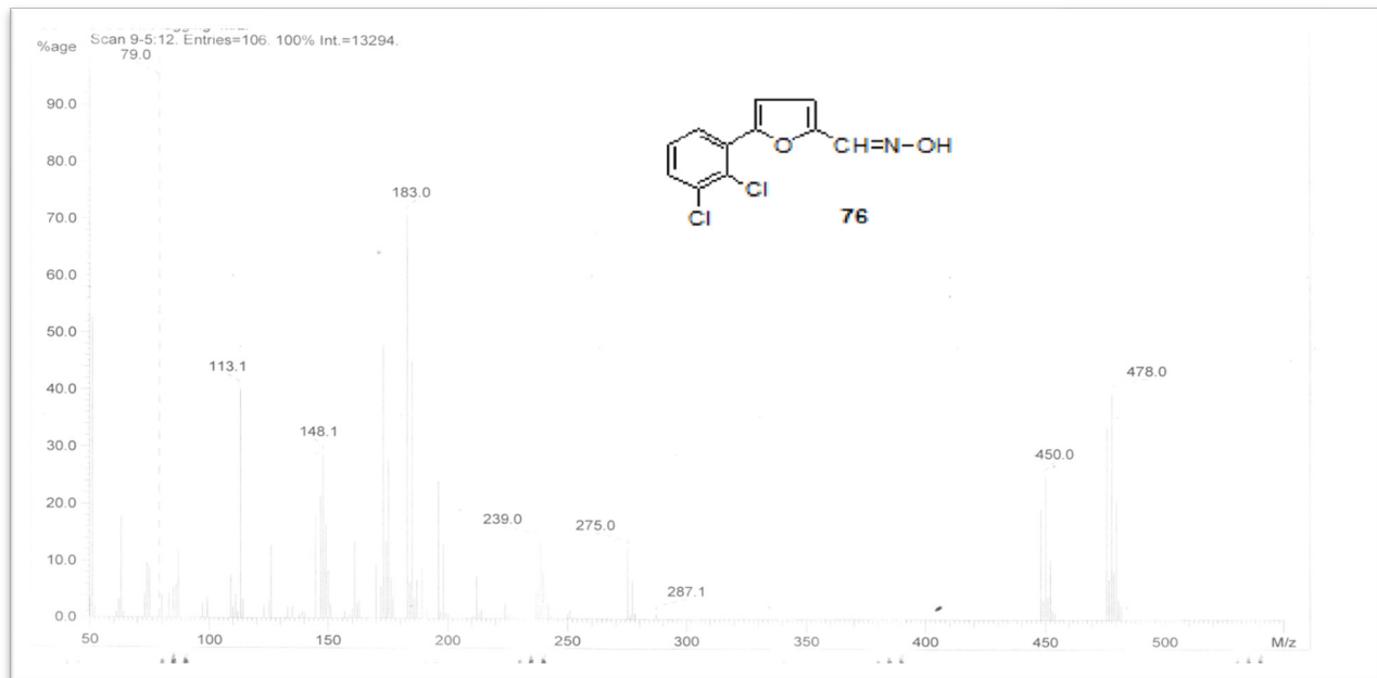
Mass spectra of 5-(2,3-dichlorophenyl) furan-2-carbaldehyde oxime: (14)
