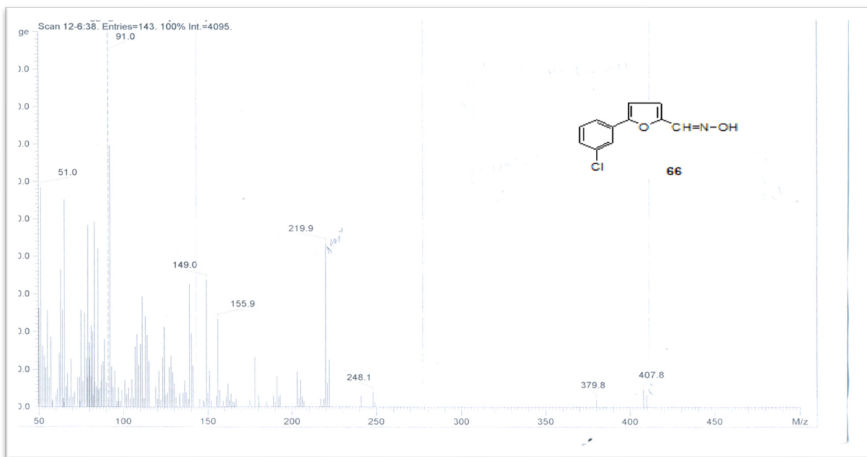
Mass spectra of 5-(3'-chlorophenyl) furan-2-carbaldehyde oxime: (5)
