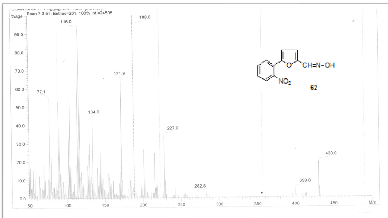
Mass spectra of 5-(2'-nitrophenyl)furan-2-carbaldehyde oxime: (1)
