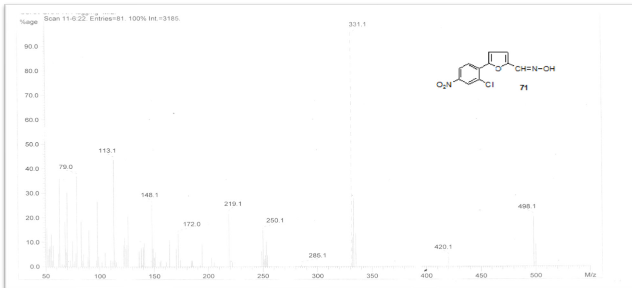
Mass spectra of 5-(2'-chloro-4'-nitrophenyl) furan-2-carbaldehyde oxime: (10)
