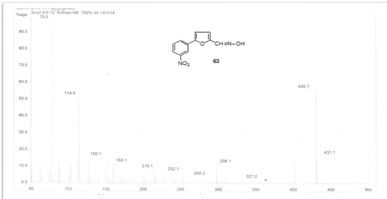
Mass spectra of 5-(3'-nitrophenyl)furan-2-carbaldehyde oxime: (2)
