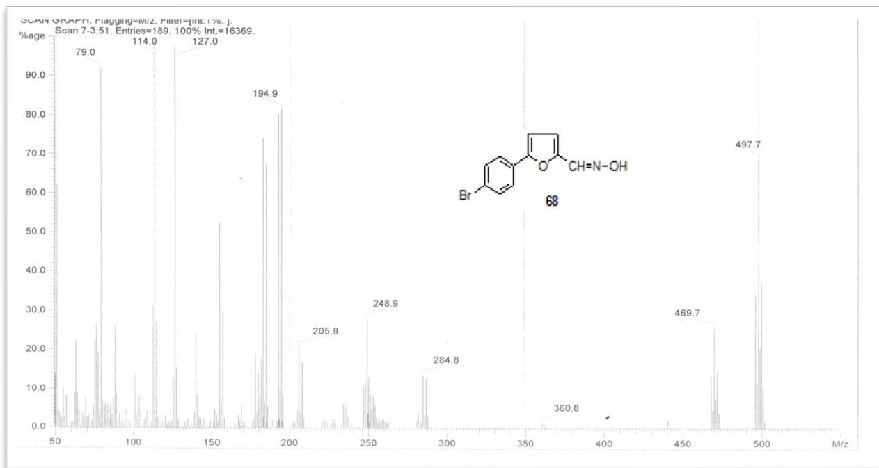
Mass spectra of 5-(4'-bromophenyl) furan-2-carbaldehyde oxime: (7)
