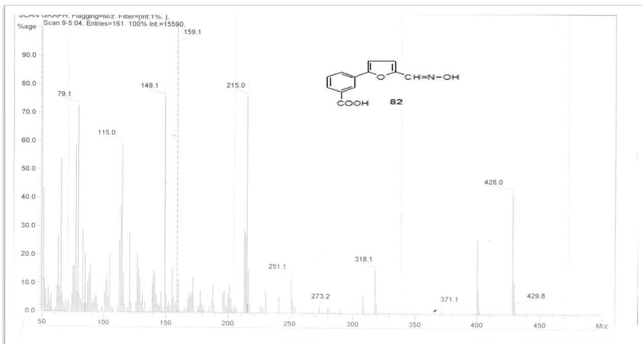
Mass spectra of 3-(5-formylfuran-2-yl)benzoic acid oxime (19)
