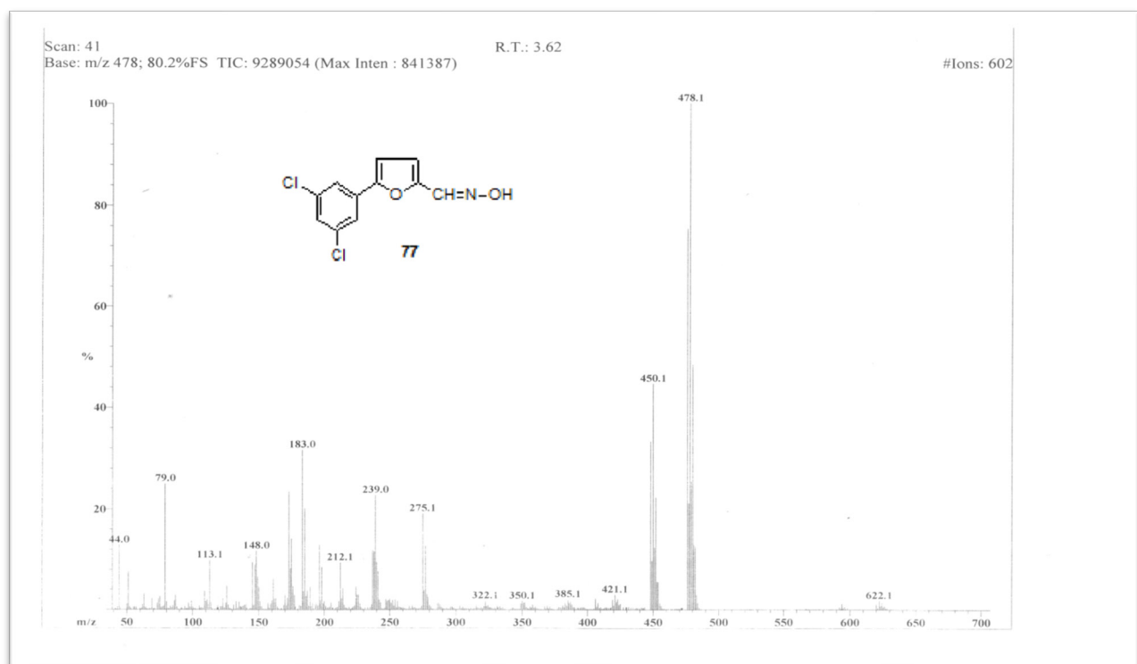
Mass spectra of 5-(3,5-dichlorophenyl) furan-2-carbaldehyde oxime: (15)
