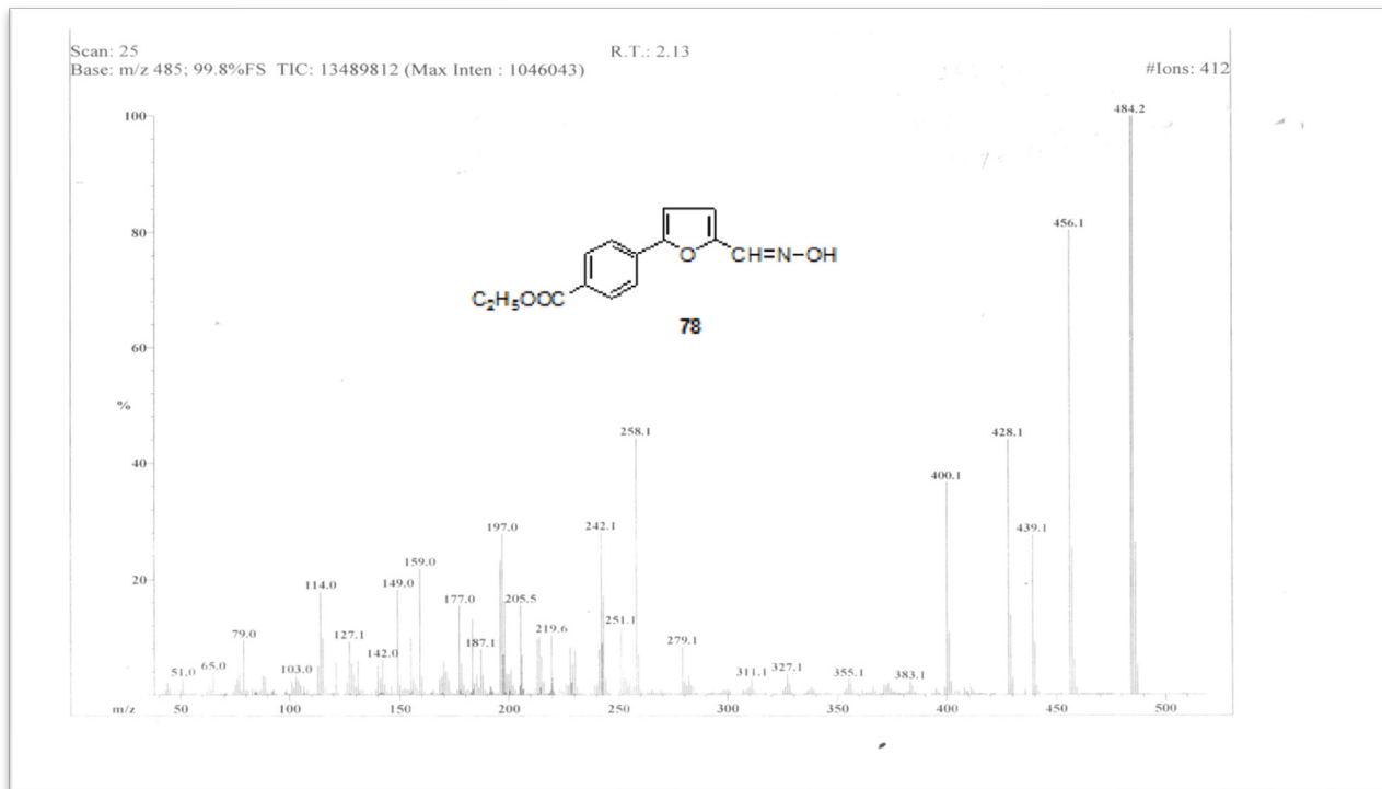
Mass spectra of 5-(4'Ethyl benzoate) furan-2-carbaldehyde oxime: (16)
