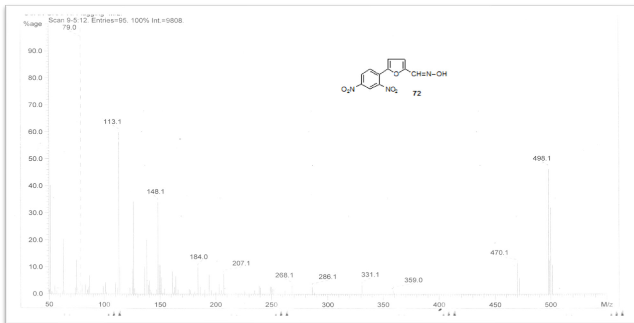
Mass spectra of 5-(2',4'-dinitrophenyl) furan-2-carbaldehyde oxime: (11)
