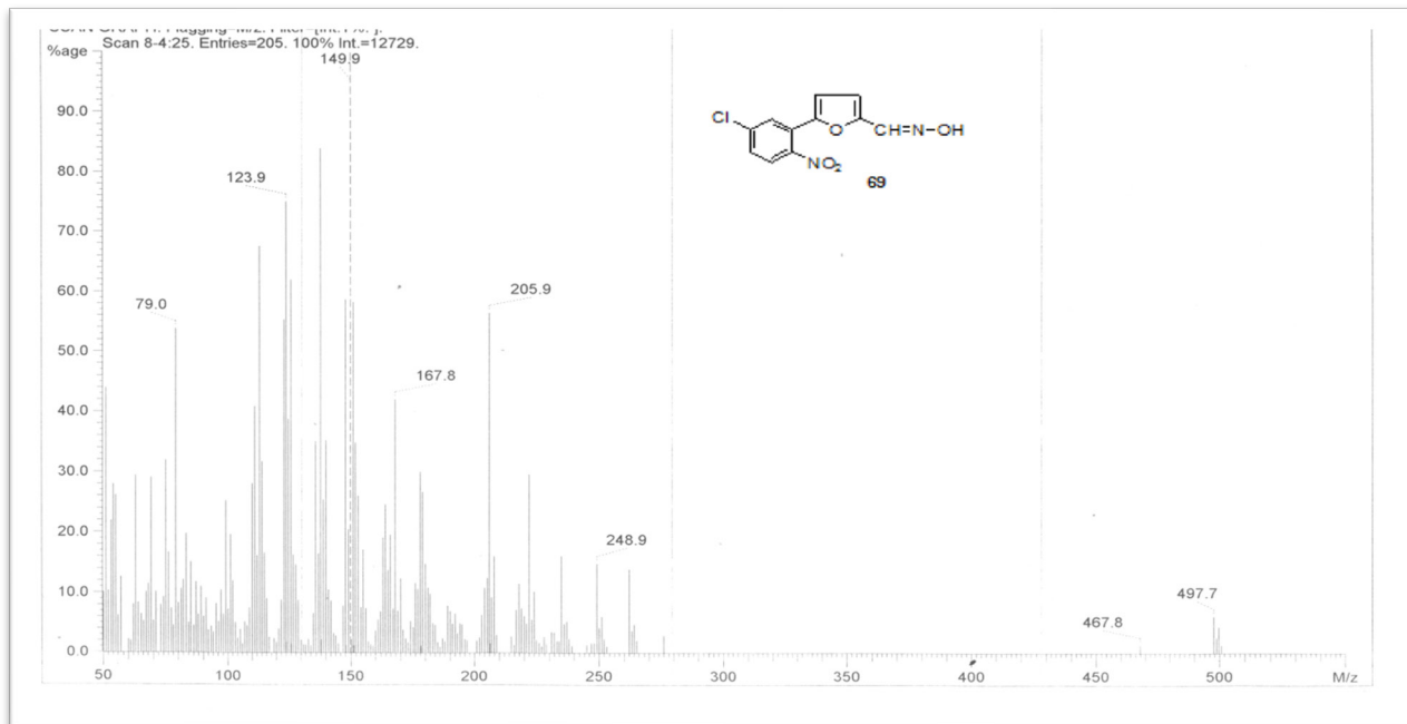
Mass spectra of 5-(5'-chloro-2'-nitrophenyl) furan-2-carbaldehyde oxime (8)
